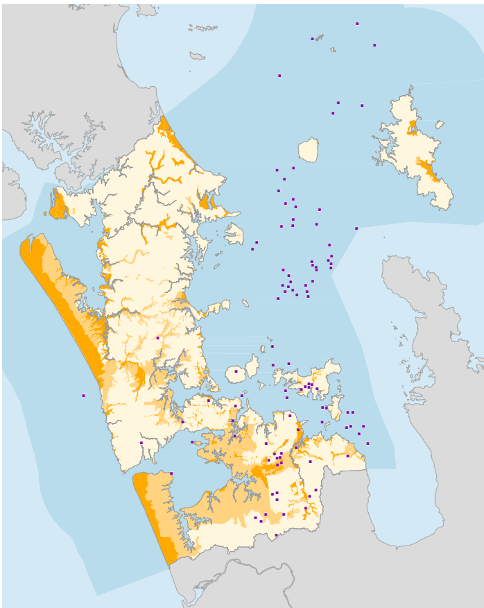
GROUND-SHAKING HAZARD
